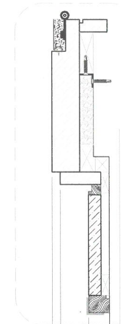
1240 30 Type A and A mir. architrave
