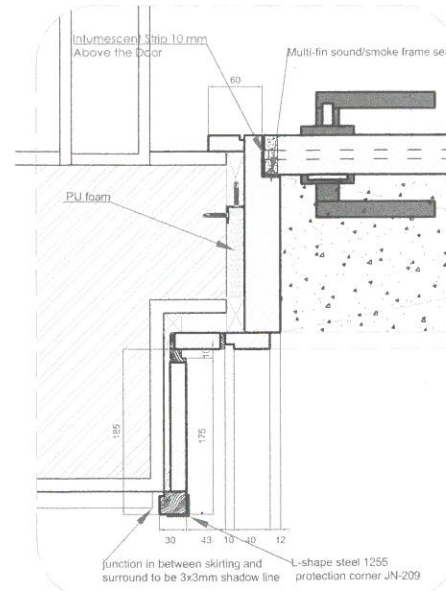
D2 Typical Frame detail
